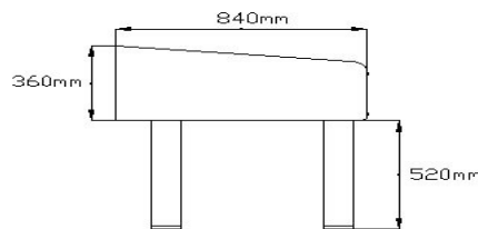
4-Head Wok Bench CookTop 2400mmW*840mmD*880mmH
