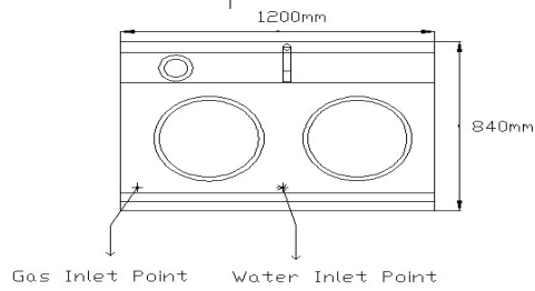
2-Head Wok Bench CookTop 1200mmW*840mmD*880mmH
