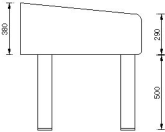
Single Wok Burner 600Wx830Dx820mmH
