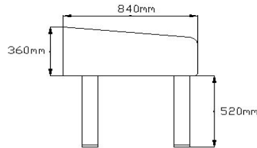
3-Head Wok Bench CookTop 1800mmW*840mmD*880mmH
