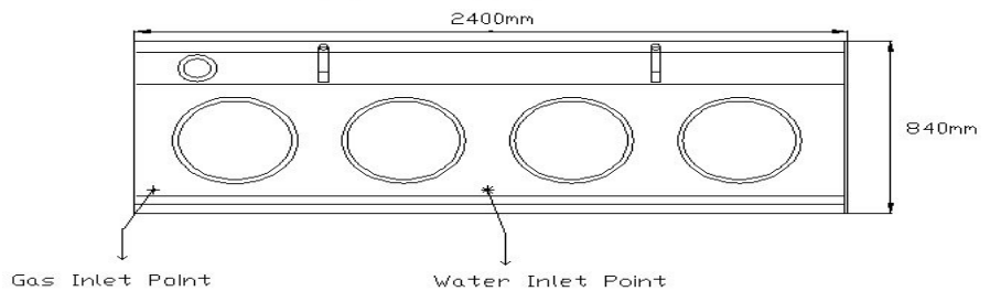
4-Head Wok Bench CookTop 2400mmW*840mmD*880mmH
